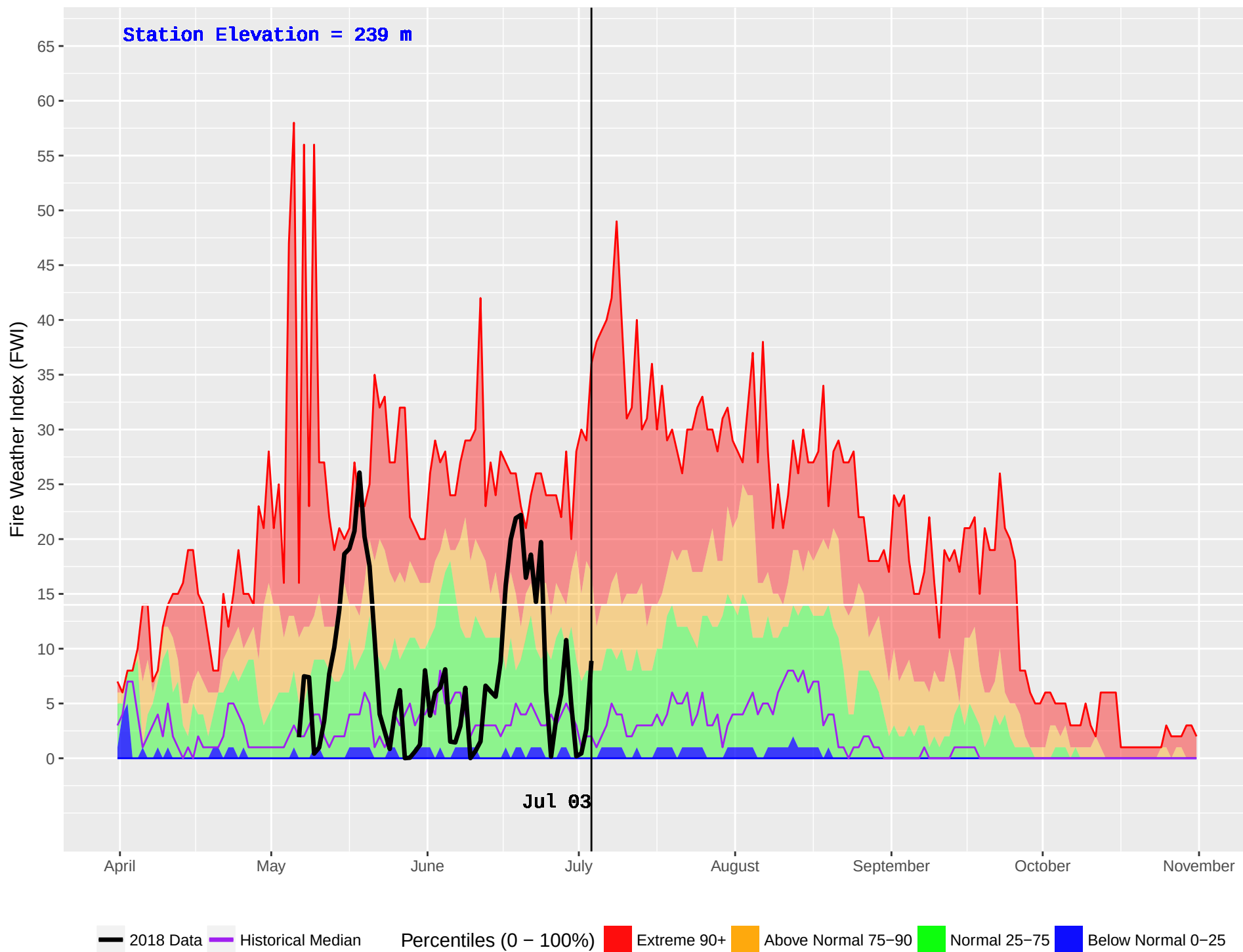
ROSSWOOD (105) : Historical (1970–2016) and Current (2018) Noon Fire Weather Index (FWI)
