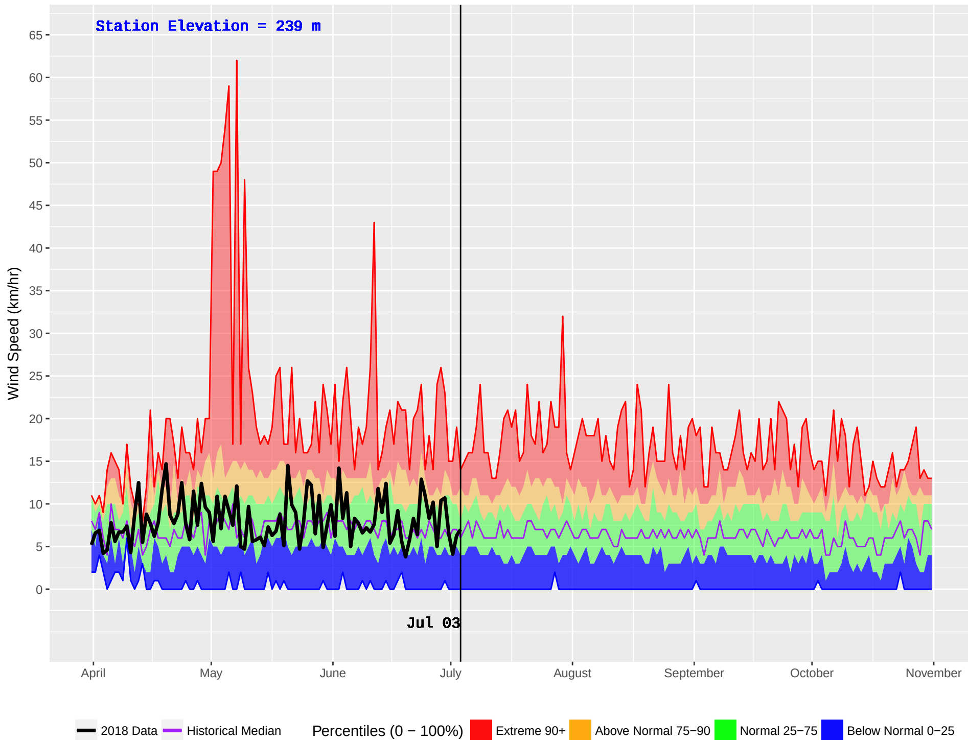
ROSSWOOD (105) : Historical (1970–2016) and Current (2018) Noon Wind Speed
