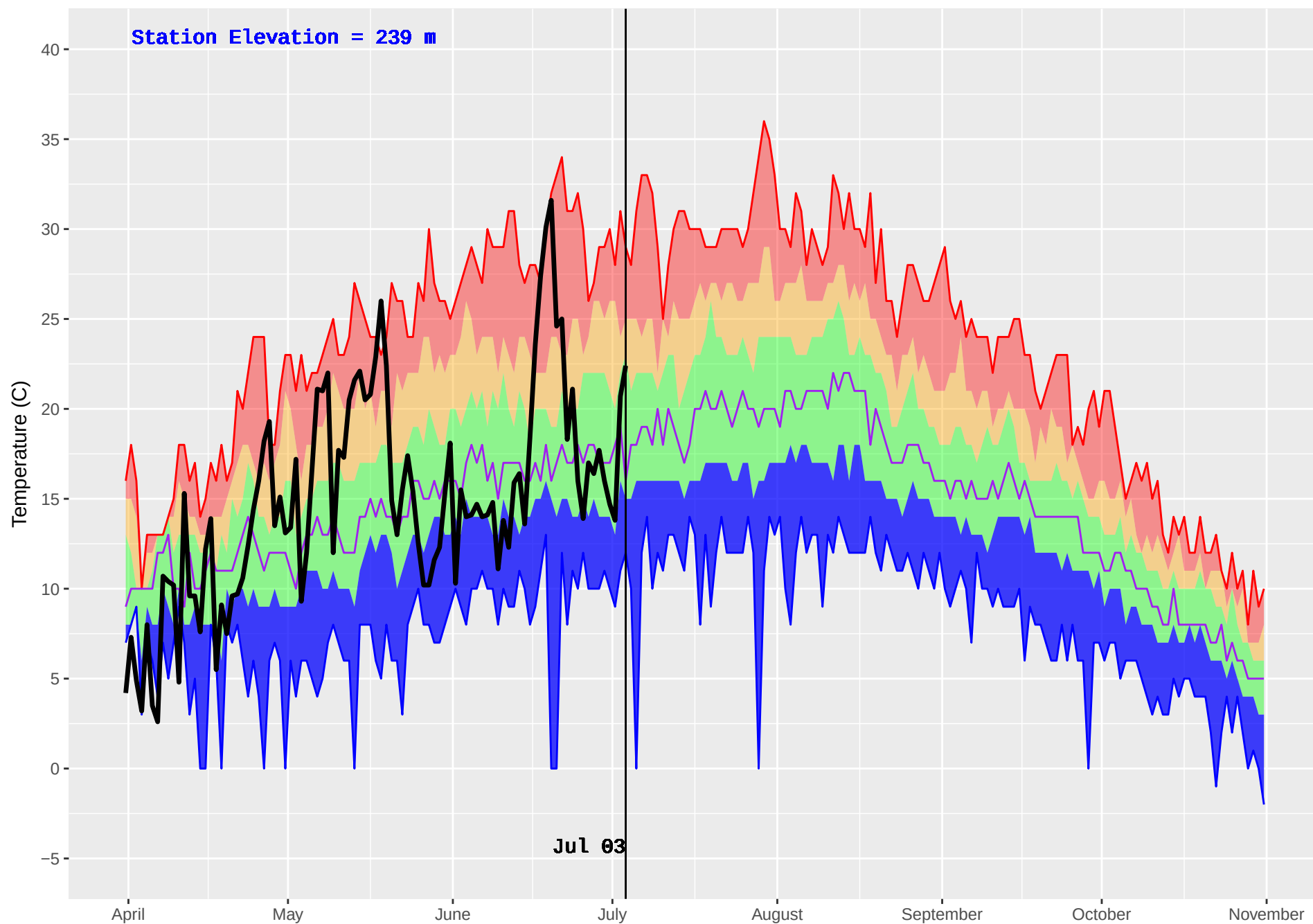
ROSSWOOD (105) : Historical (1970–2016) and Current (2018) Noon Temperature
