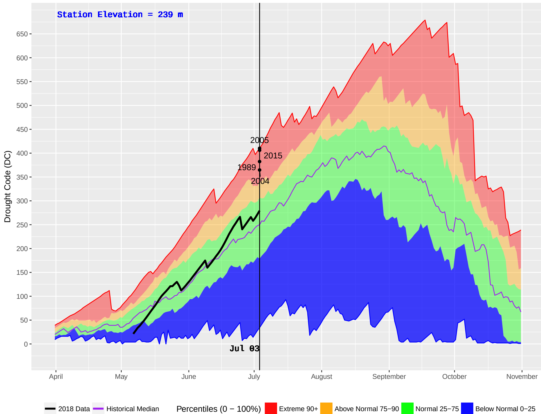
ROSSWOOD (105) : Historical (1970–2016) and Current (2018) Noon Drought Code (DC)
