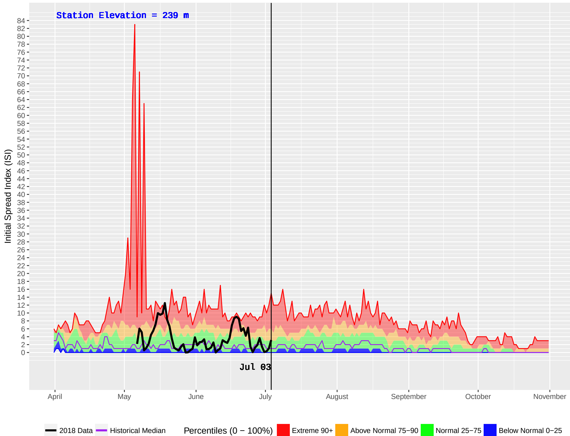
ROSSWOOD (105) : Historical (1970–2016) and Current (2018) Noon Initial Spread Index (ISI)
