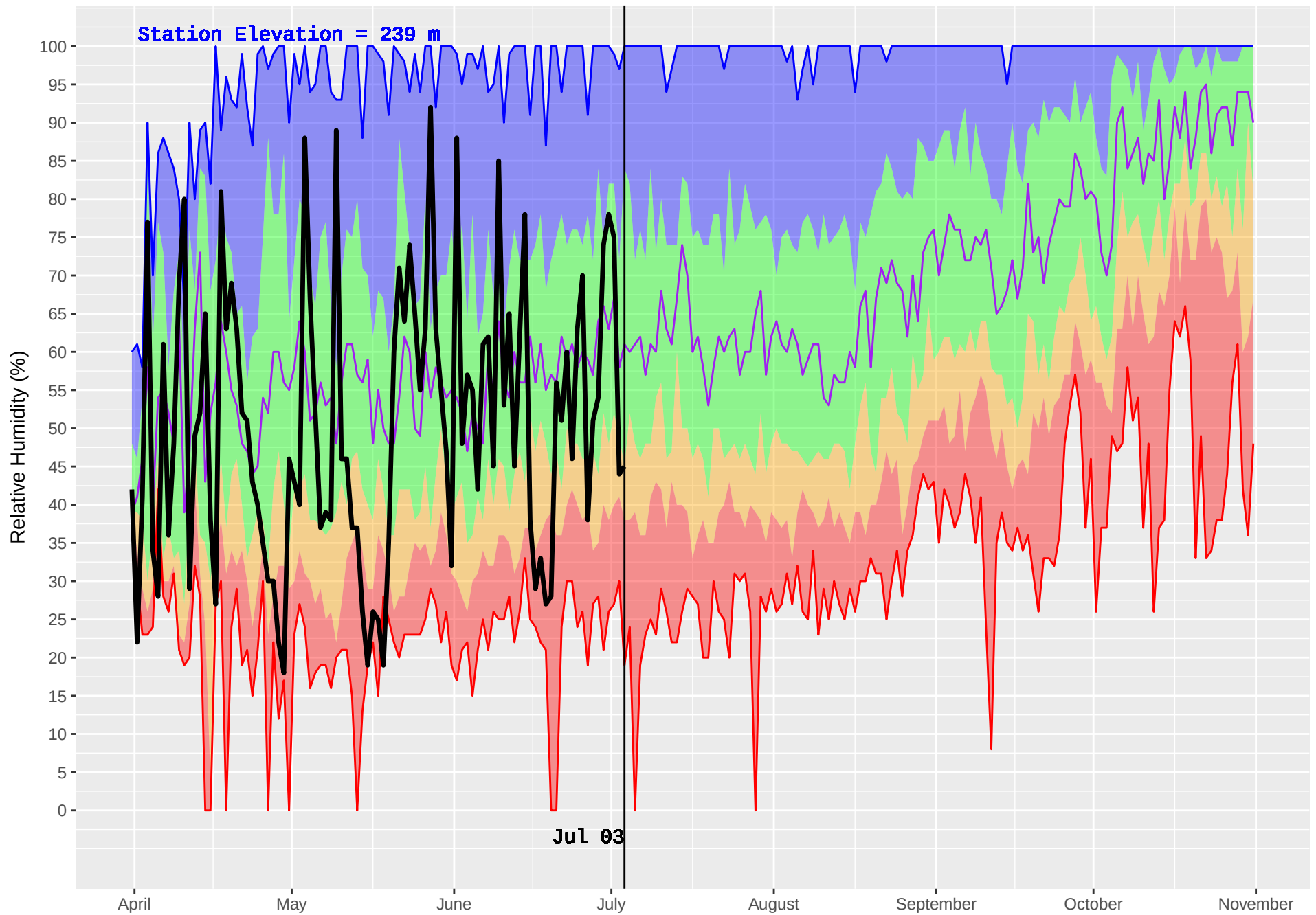
ROSSWOOD (105) : Historical (1970–2016) and Current (2018) Noon Relative Humidity
