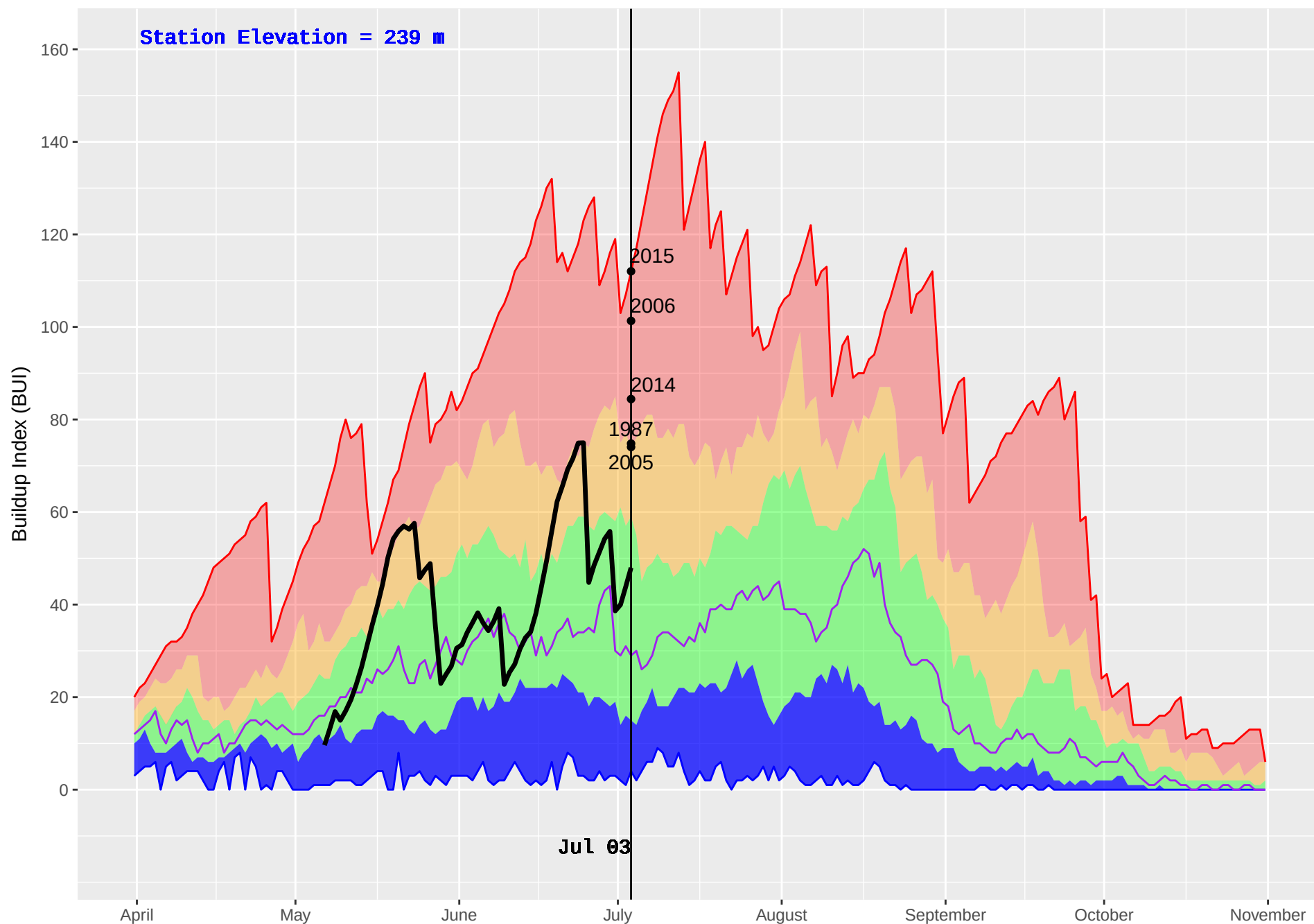
ROSSWOOD (105) : Historical (1970–2016) and Current (2018) Noon Buildup Index (BUI)
